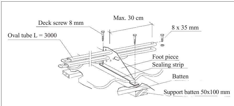
Drawing 17 Snow barrier fastening
