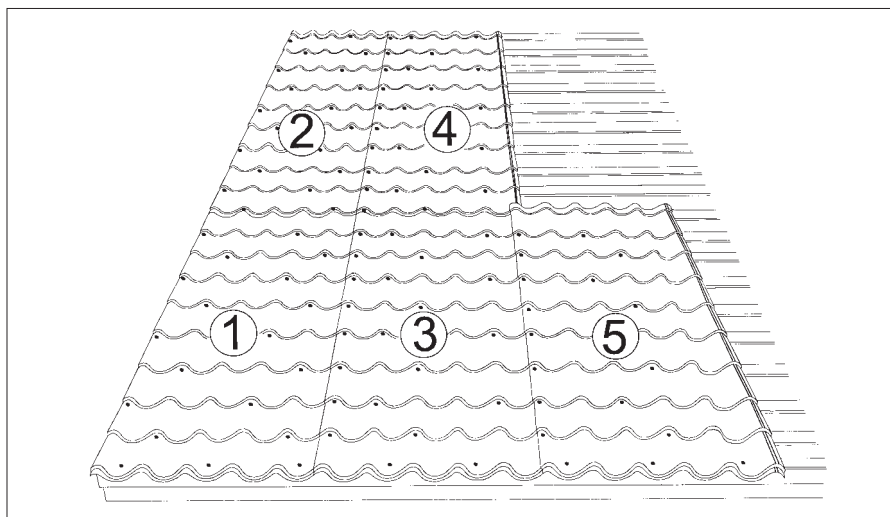
Drawing 12 Installation order and spacing between screws
