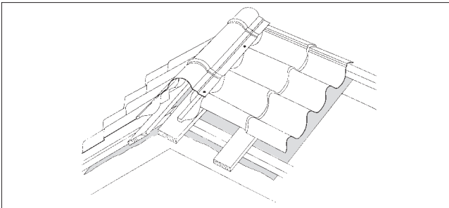
Drawing 10 Ridge structure
