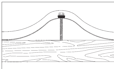
Drawing 13 Fastening to roof board
