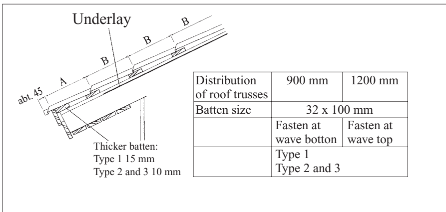
Drawing 5 Roof board dimensioning
