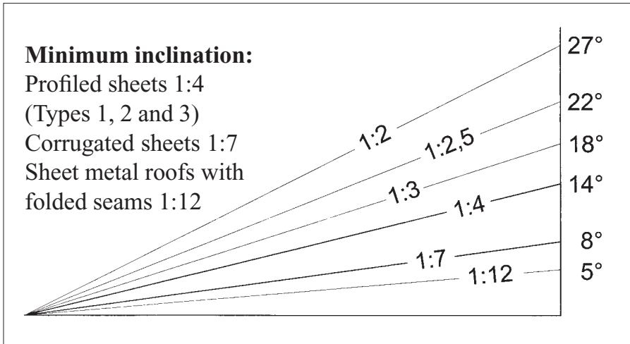
Drawing 18 Minimum inclination
