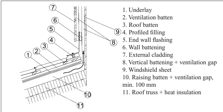
Drawing 9 Roof and wall joint
