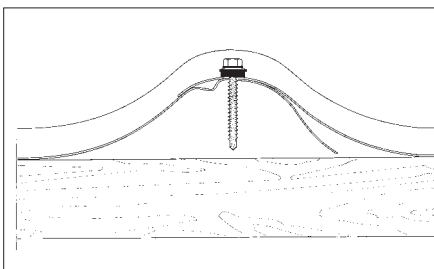
Drawing 14 Lateral overlap
