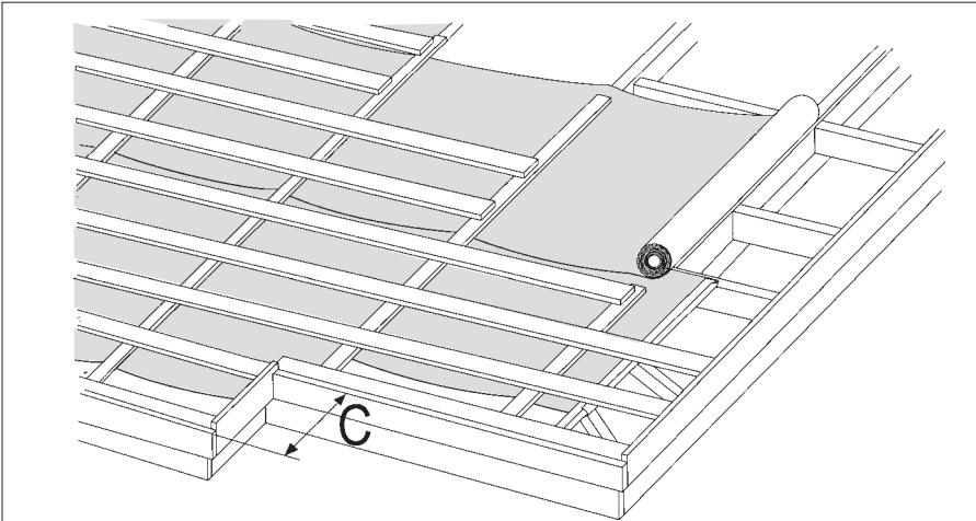
Drawing 4 Construction drawing for installation of underlay
