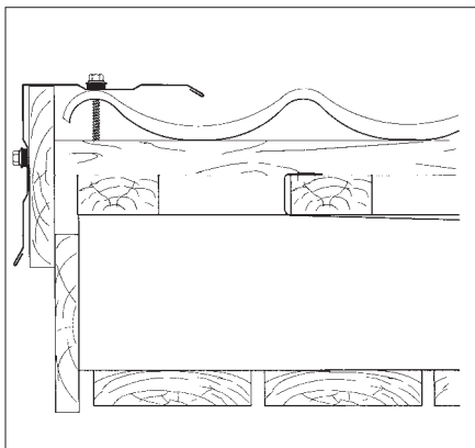
Drawing 6 Gable eaves
