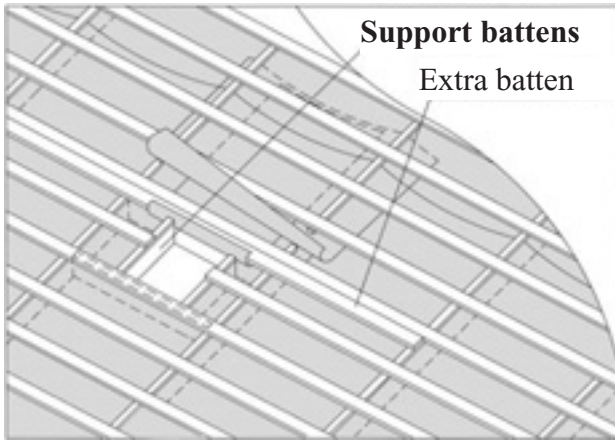
Drawing 11 Thru hole supports
