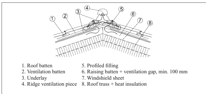
Drawing 8 Ridge ventilation piece
